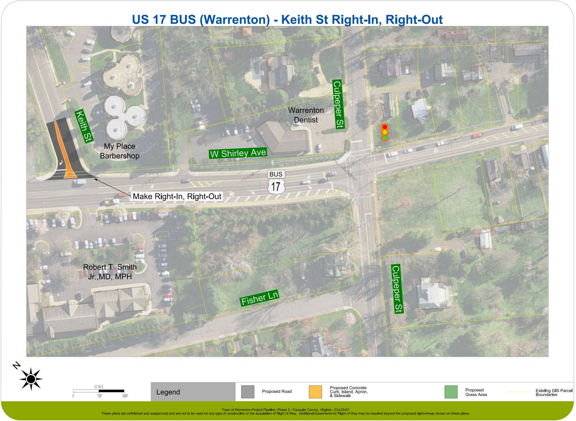
Figure 2-5: Keith Street Right-In, Right-Out Layout
