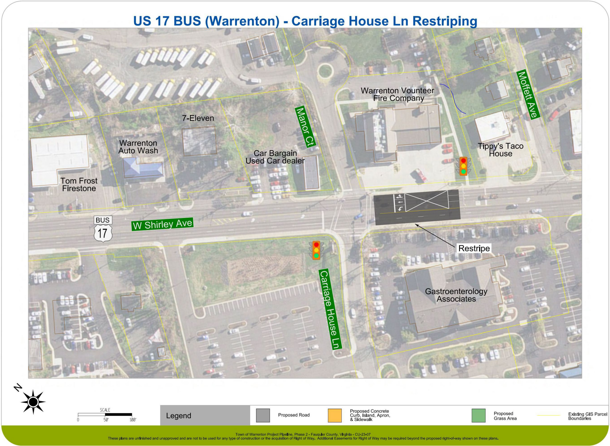
Figure 2-4: Carriage House Lane Restriping
